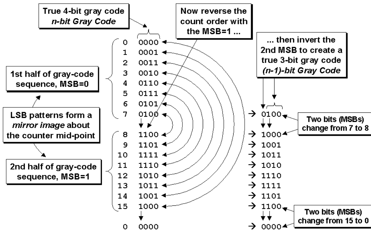
Figure 2 - n -bit Gray code converted to an (n-1) -bit Gray code
