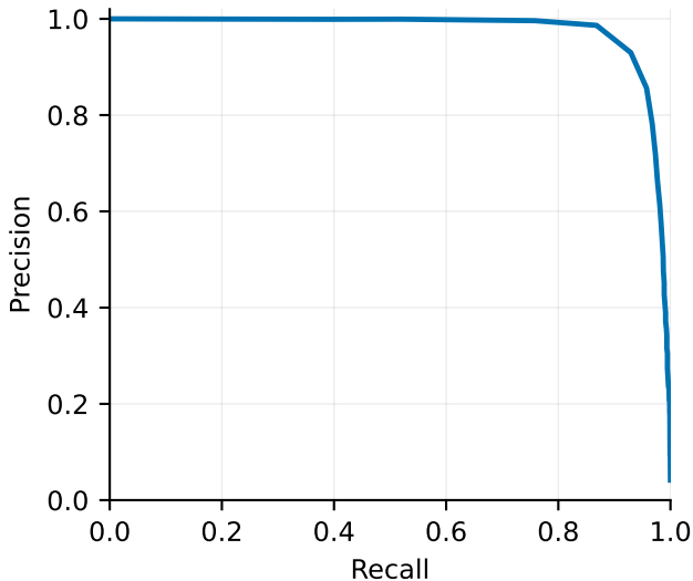
Custom CNN (v2) — segment-level Precision-Recall (micro-average)
