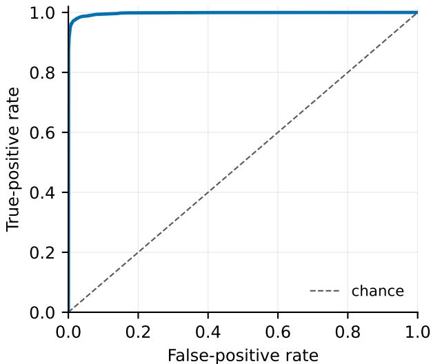
Custom CNN (v2) — segment-level ROC (micro-average)
