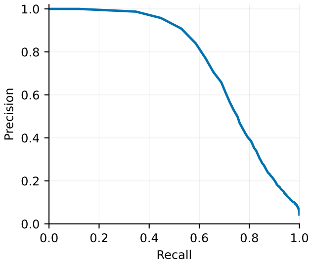
Custom CNN (v4) — recording-level Precision-Recall (micro-average)
