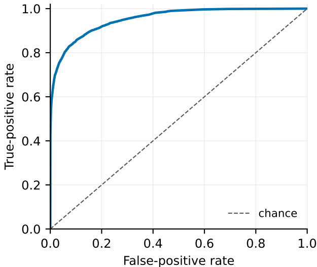
Custom CNN (v4) — recording-level ROC (micro-average)
