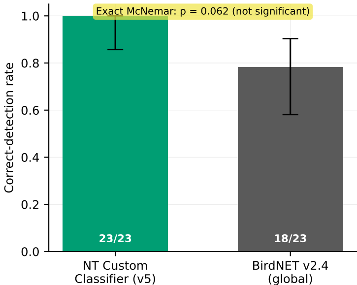
NT model vs global BirdNET on 23 shared recordings (Wilson 95% CIs)
