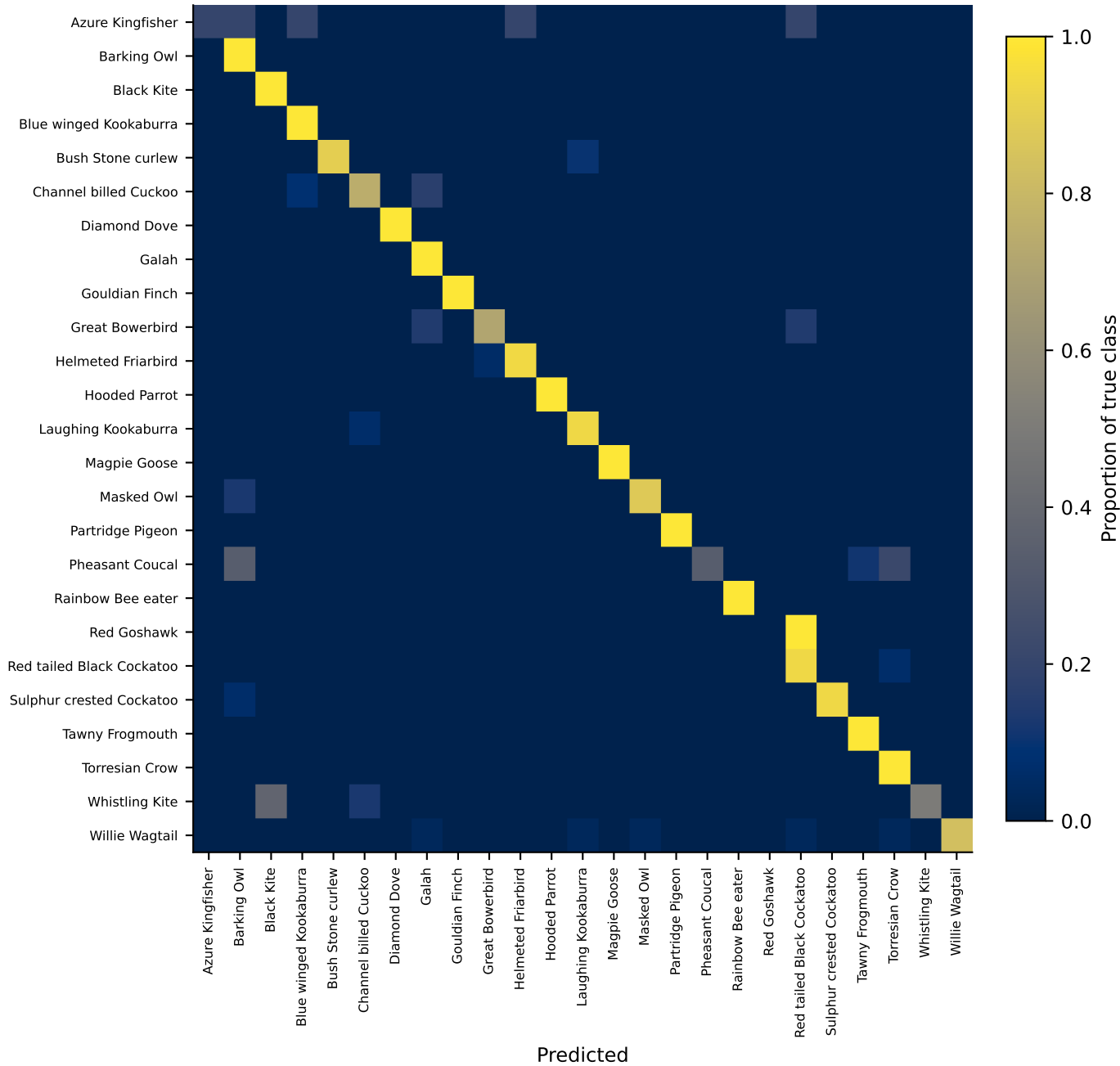
NT Custom Classifier (v5) — recording-level held-out Row-normalised confusion matrix
