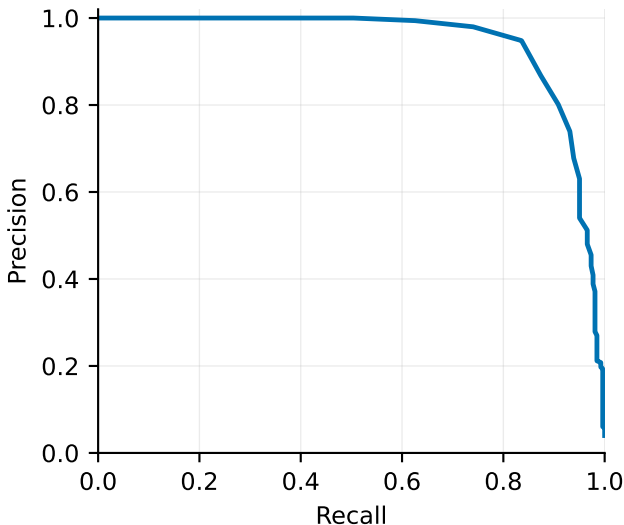
NT Custom Classifier (v5) — recording-level held-out Precision-Recall (micro-average)
