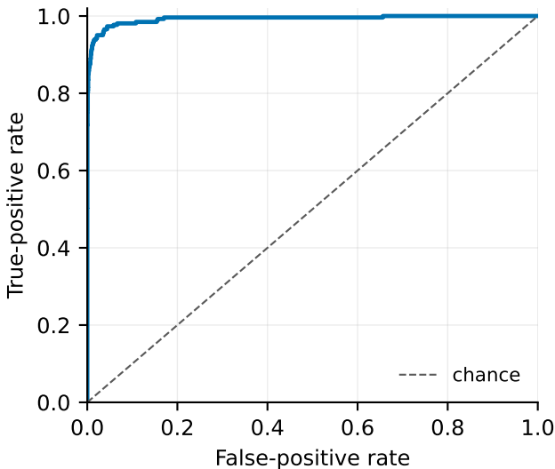
NT Custom Classifier (v5) — recording-level held-out ROC (micro-average)
