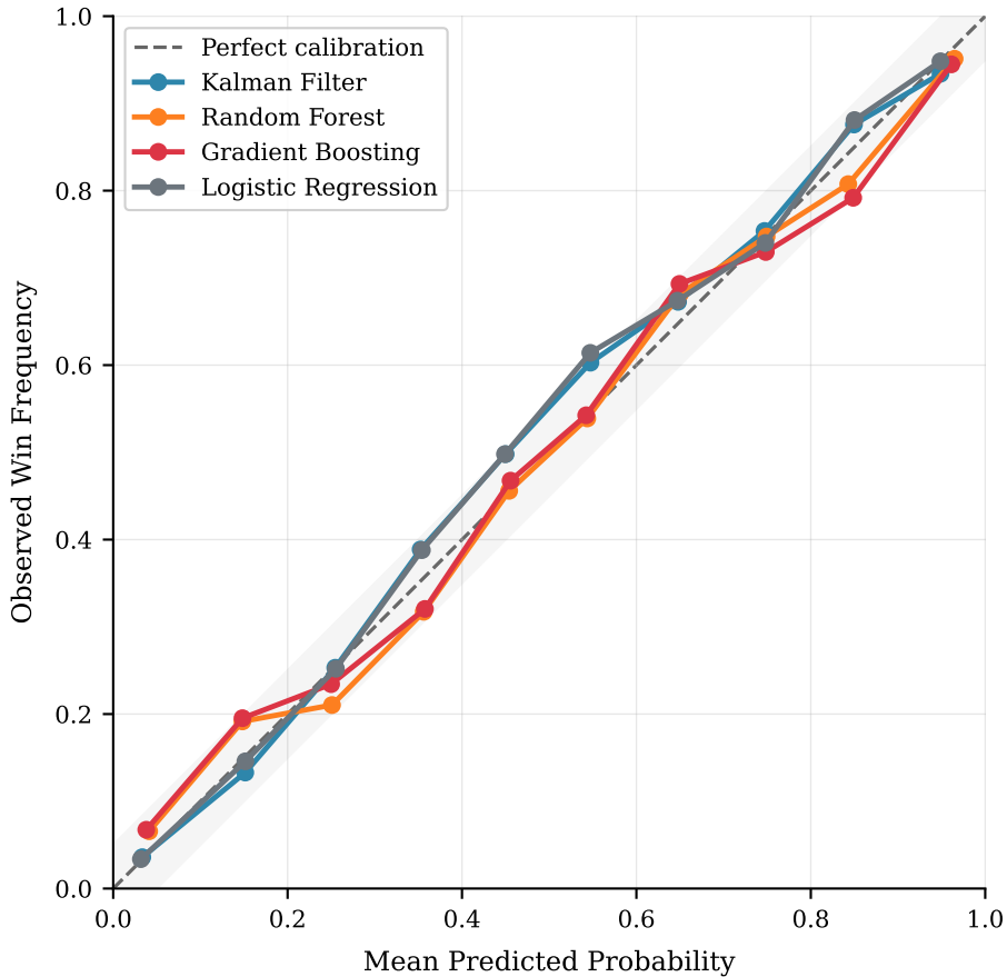
Reliability Diagram (Calibration Curves)
