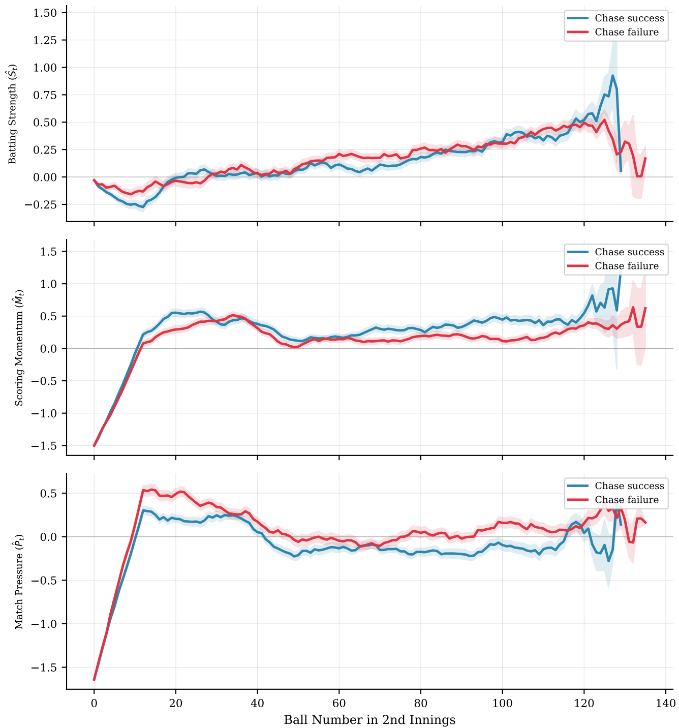
Mean Filtered Latent States: Successful vs. Failed Chases (Shaded region = \pm 1 SE across matches)
