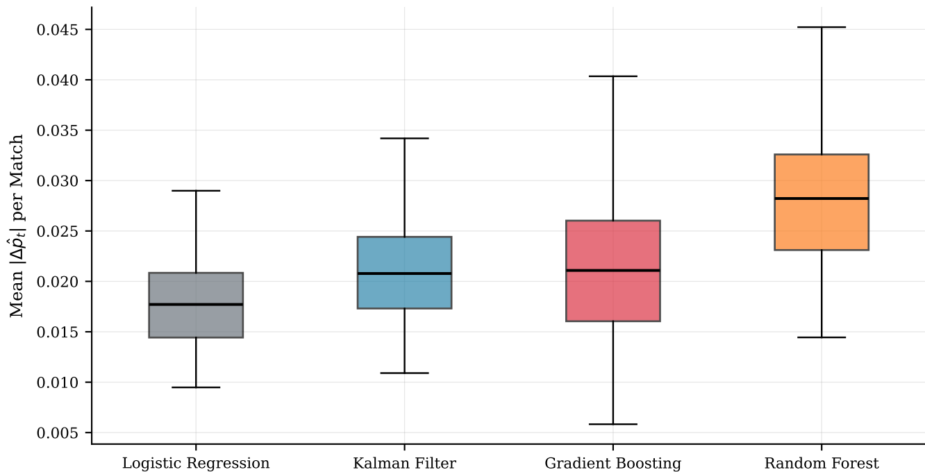
Prediction Volatility Distribution by Model
