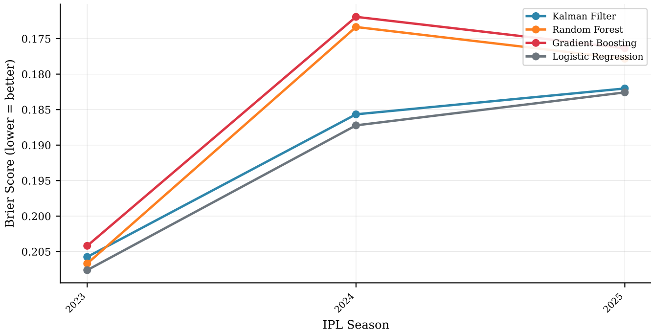
Season-by-Season Brier Score
