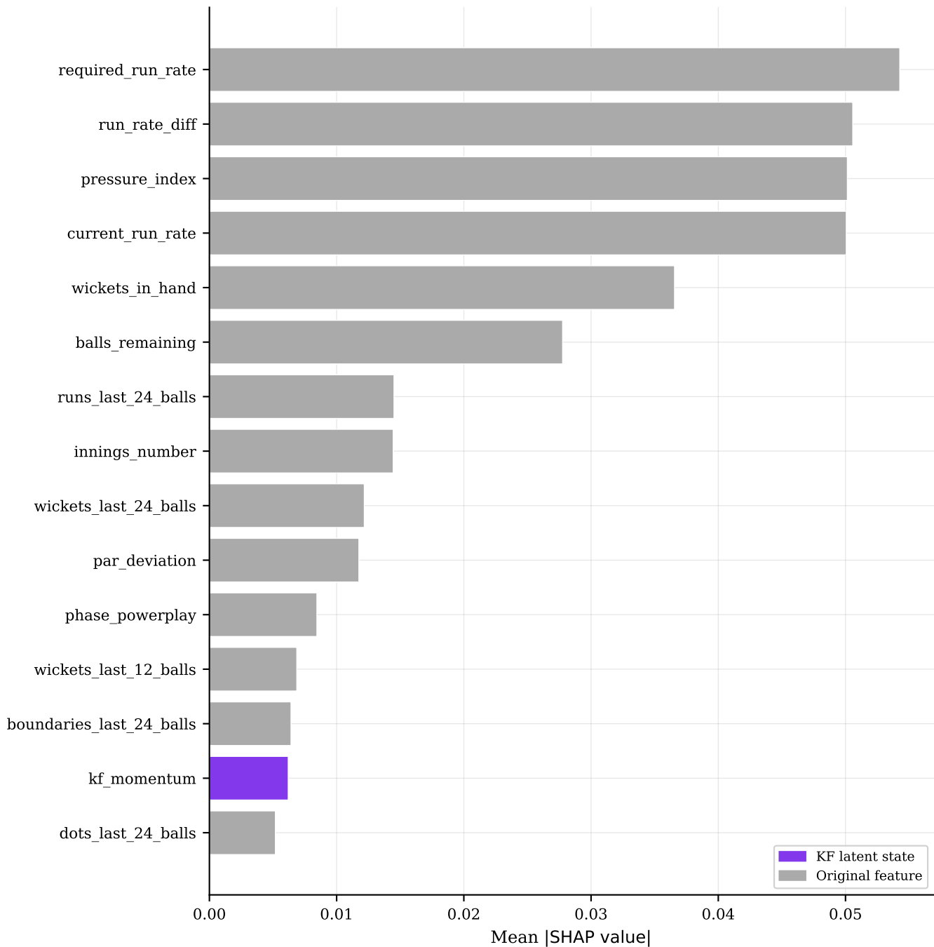
Top 15 Feature Importances — Hybrid RF+KF Model
