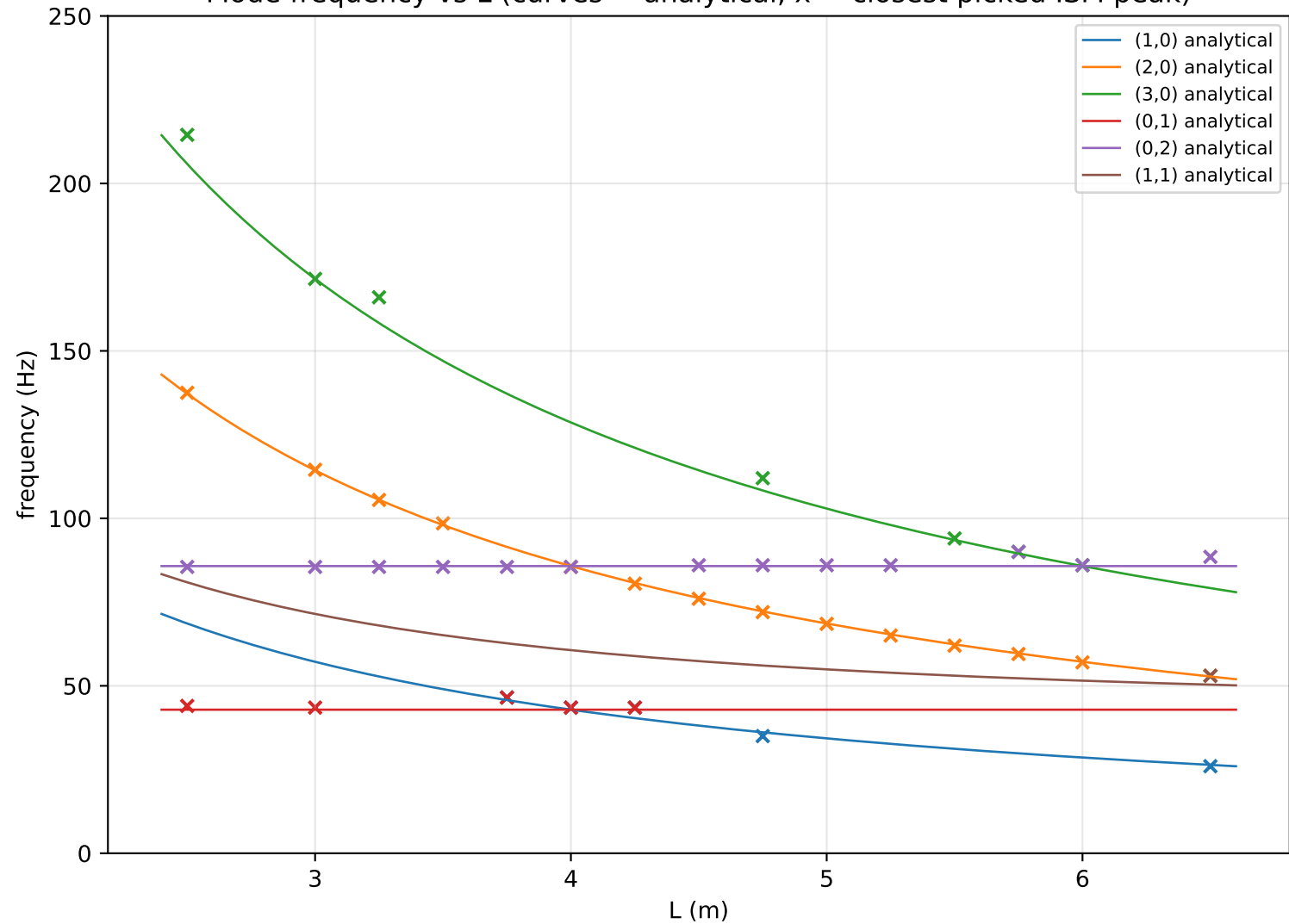
Mode frequency vs L (curves = analytical, x = closest picked ISM peak)
