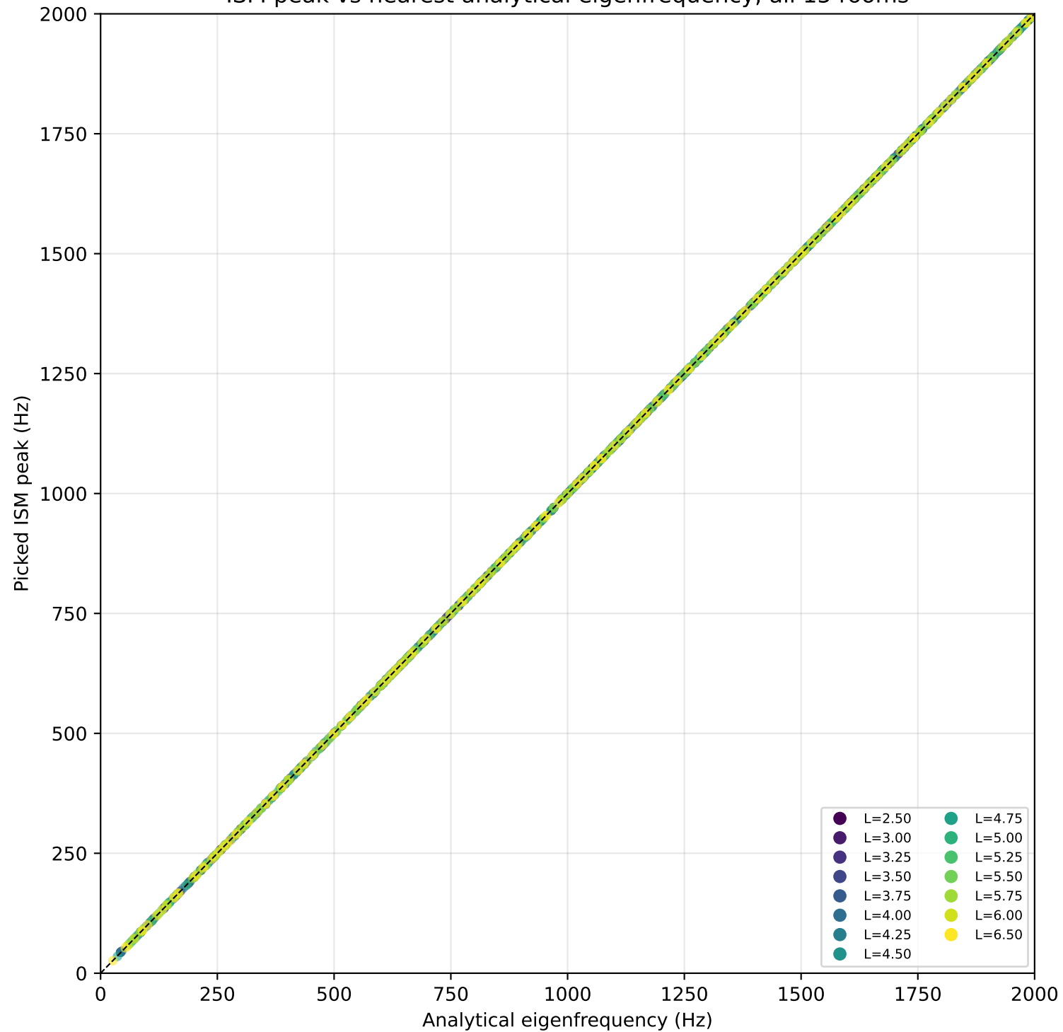
ISM peak vs nearest analytical eigenfrequency, all 15 rooms
