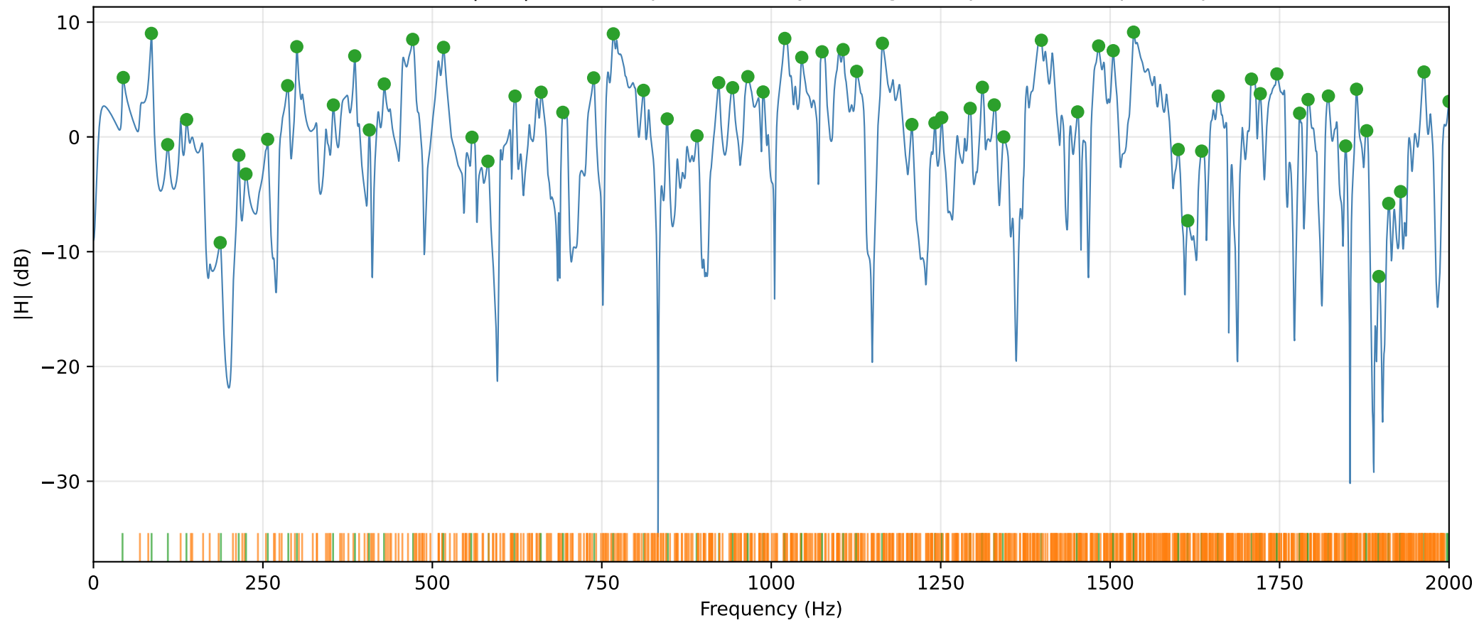
L=2.50 m — ISM |H(f)| with deduplicated analytical eigenfrequencies and picked peaks
