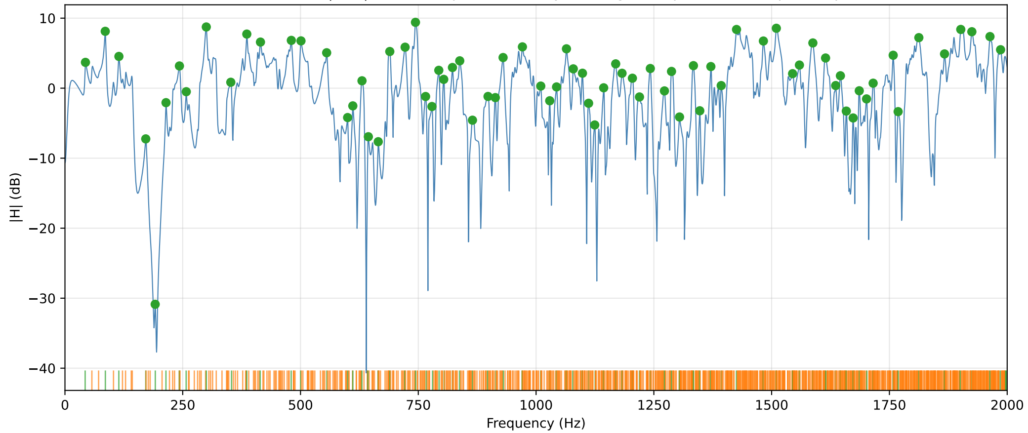
L=3.00 m — ISM |H(f)| with deduplicated analytical eigenfrequencies and picked peaks
