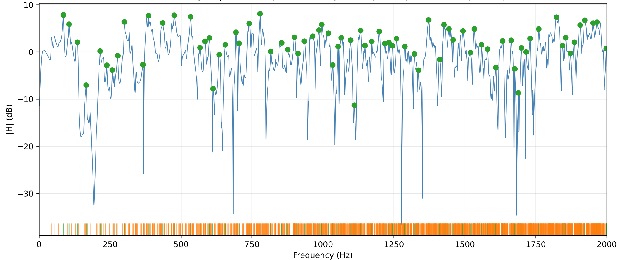
L=3.25 m — ISM |H(f)| with deduplicated analytical eigenfrequencies and picked peaks
