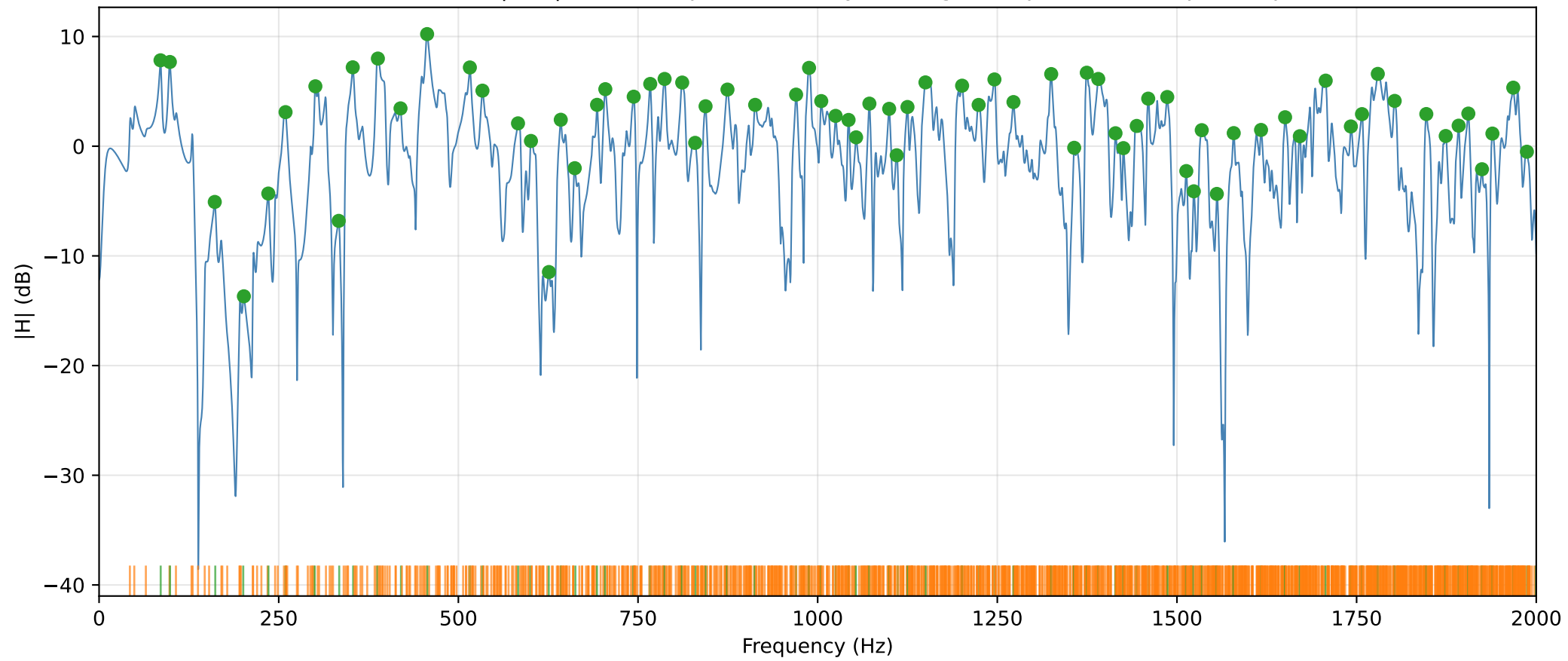
L=3.50 m — ISM |H(f)| with deduplicated analytical eigenfrequencies and picked peaks
