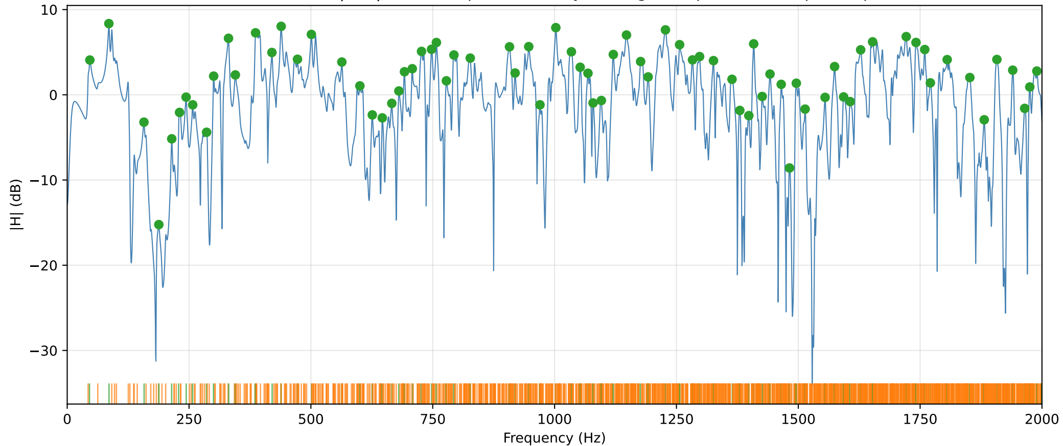
L=3.75 m — ISM |H(f)| with deduplicated analytical eigenfrequencies and picked peaks
