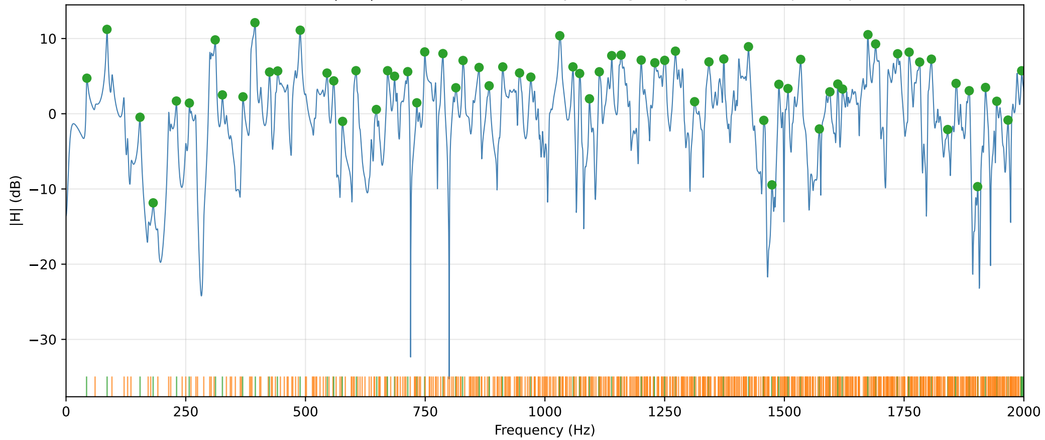
L=4.00 m — ISM |H(f)| with deduplicated analytical eigenfrequencies and picked peaks
