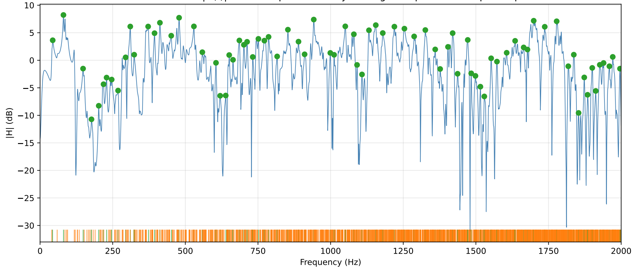
L=4.25 m — ISM |H(f)| with deduplicated analytical eigenfrequencies and picked peaks
