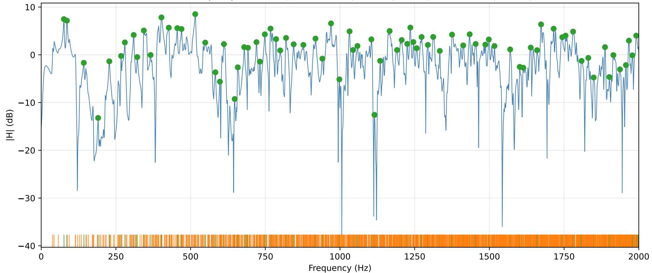
L=4.50 m — ISM |H(f)| with deduplicated analytical eigenfrequencies and picked peaks
