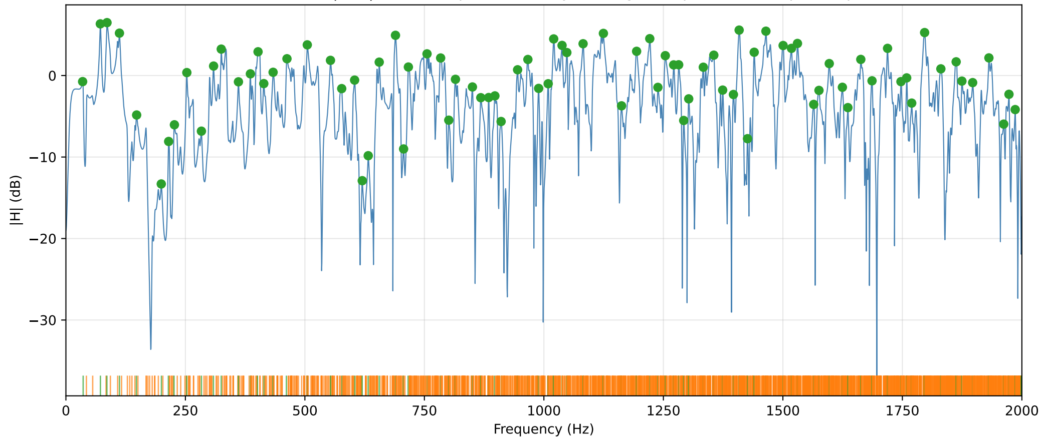
L=4.75 m — ISM |H(f)| with deduplicated analytical eigenfrequencies and picked peaks
