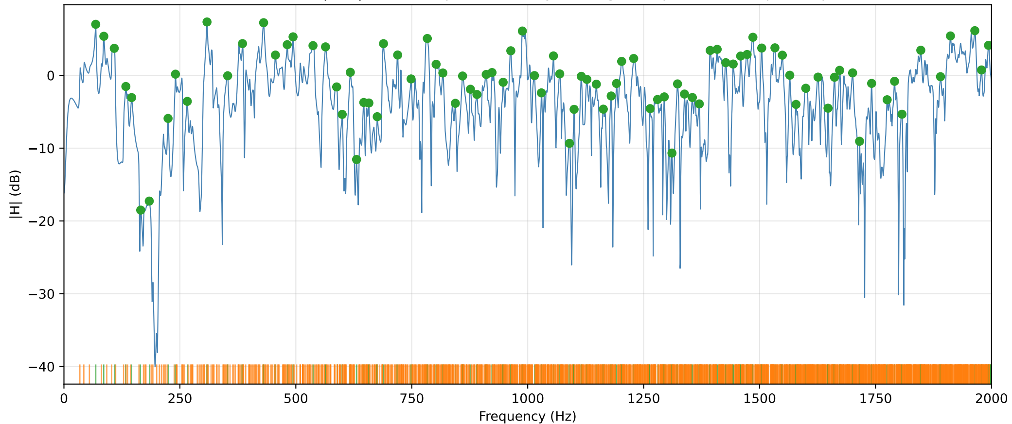
L=5.00 m — ISM |H(f)| with deduplicated analytical eigenfrequencies and picked peaks
