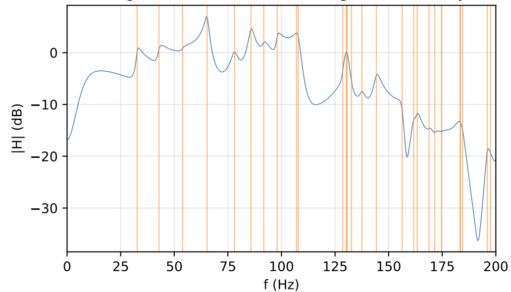
Modal-regime zoom 0-200 Hz (orange ticks = analytical)
