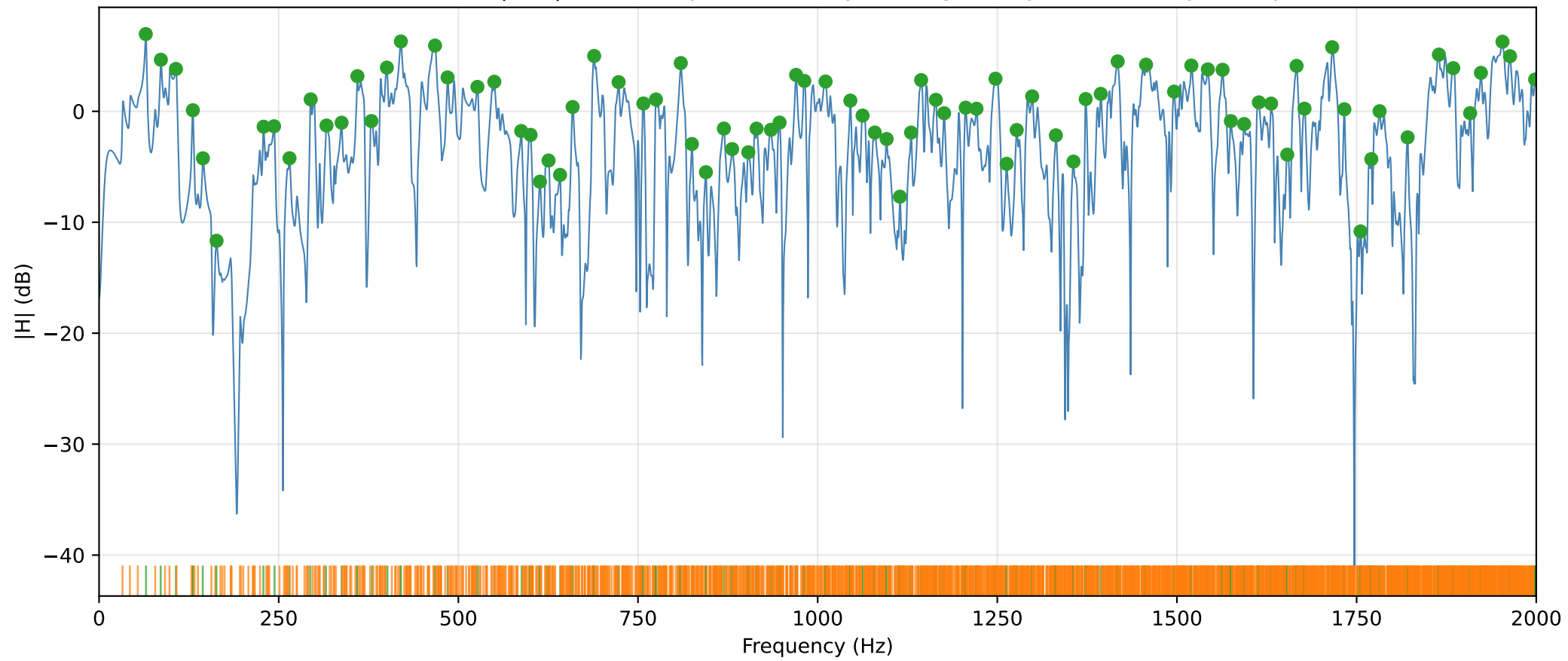
L=5.25 m — ISM |H(f)| with deduplicated analytical eigenfrequencies and picked peaks
