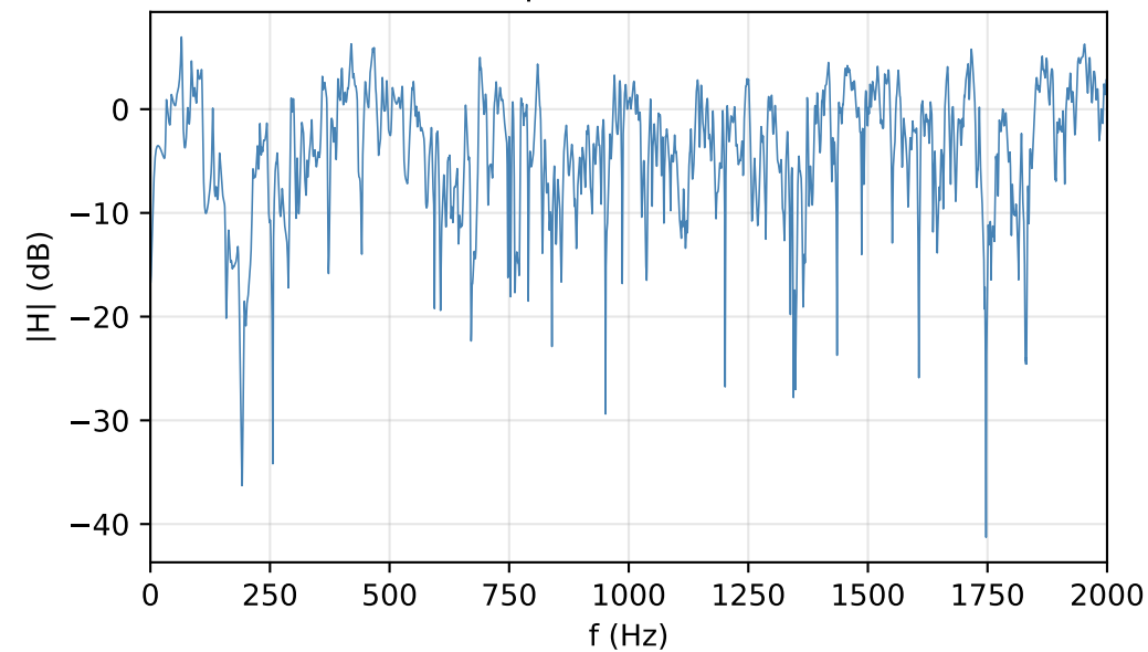
Full spectrum 0-2 kHz
