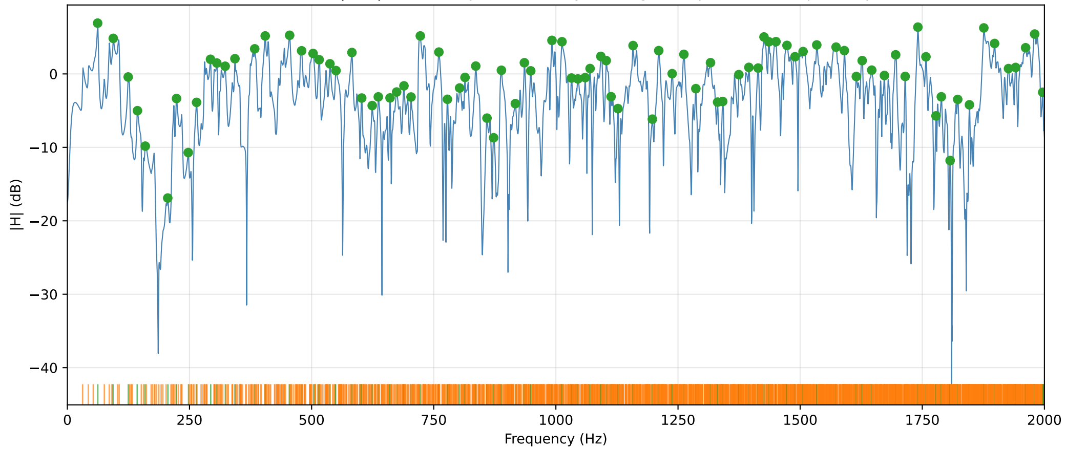
L=5.50 m — ISM |H(f)| with deduplicated analytical eigenfrequencies and picked peaks
