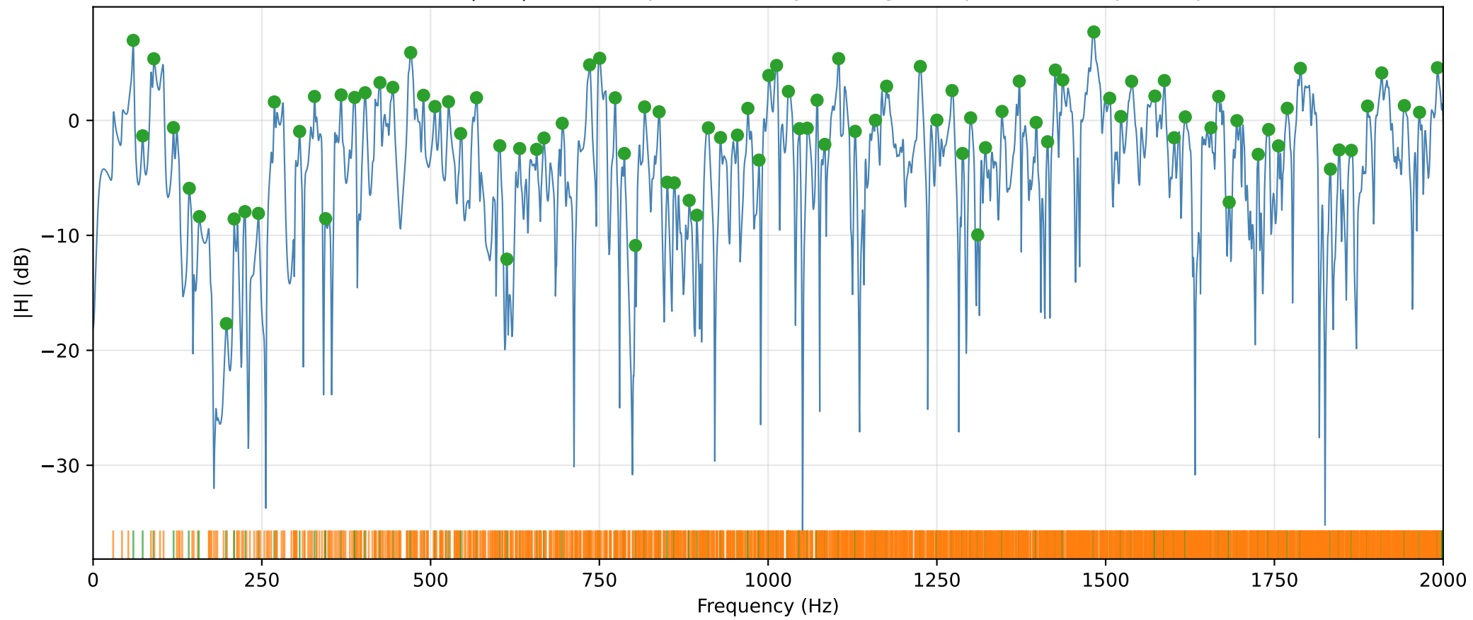
L=5.75 m — ISM |H(f)| with deduplicated analytical eigenfrequencies and picked peaks
