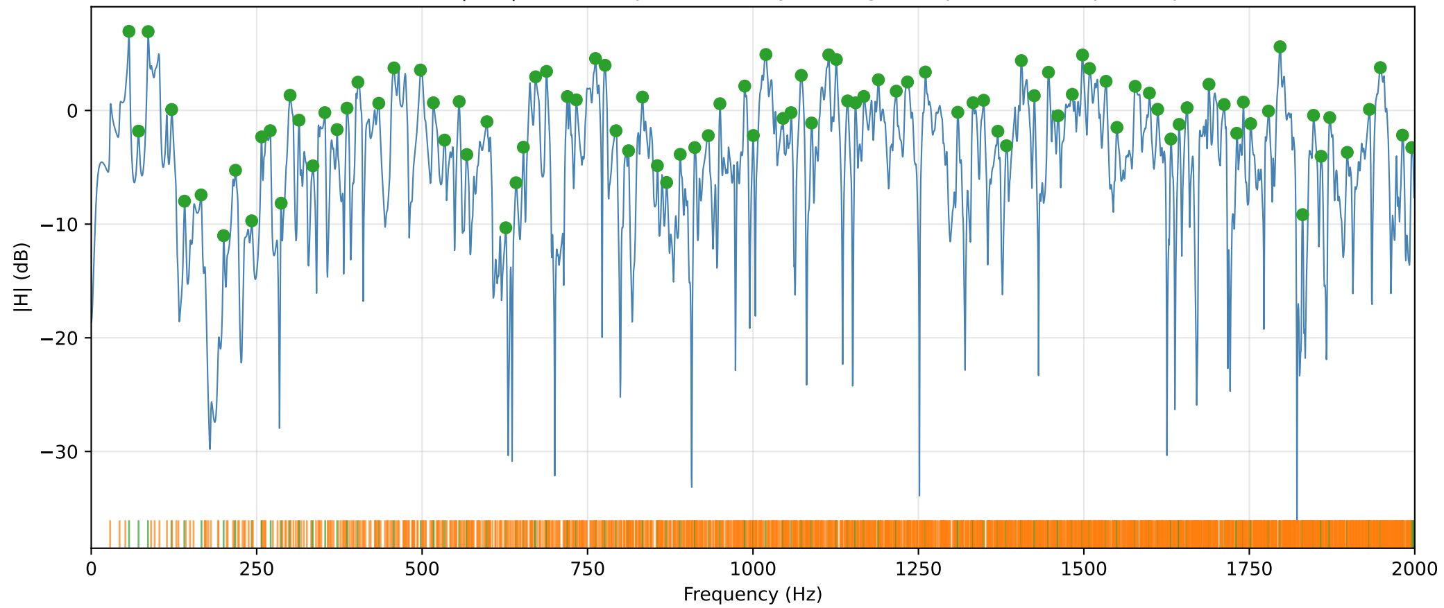
L=6.00 m — ISM |H(f)| with deduplicated analytical eigenfrequencies and picked peaks
