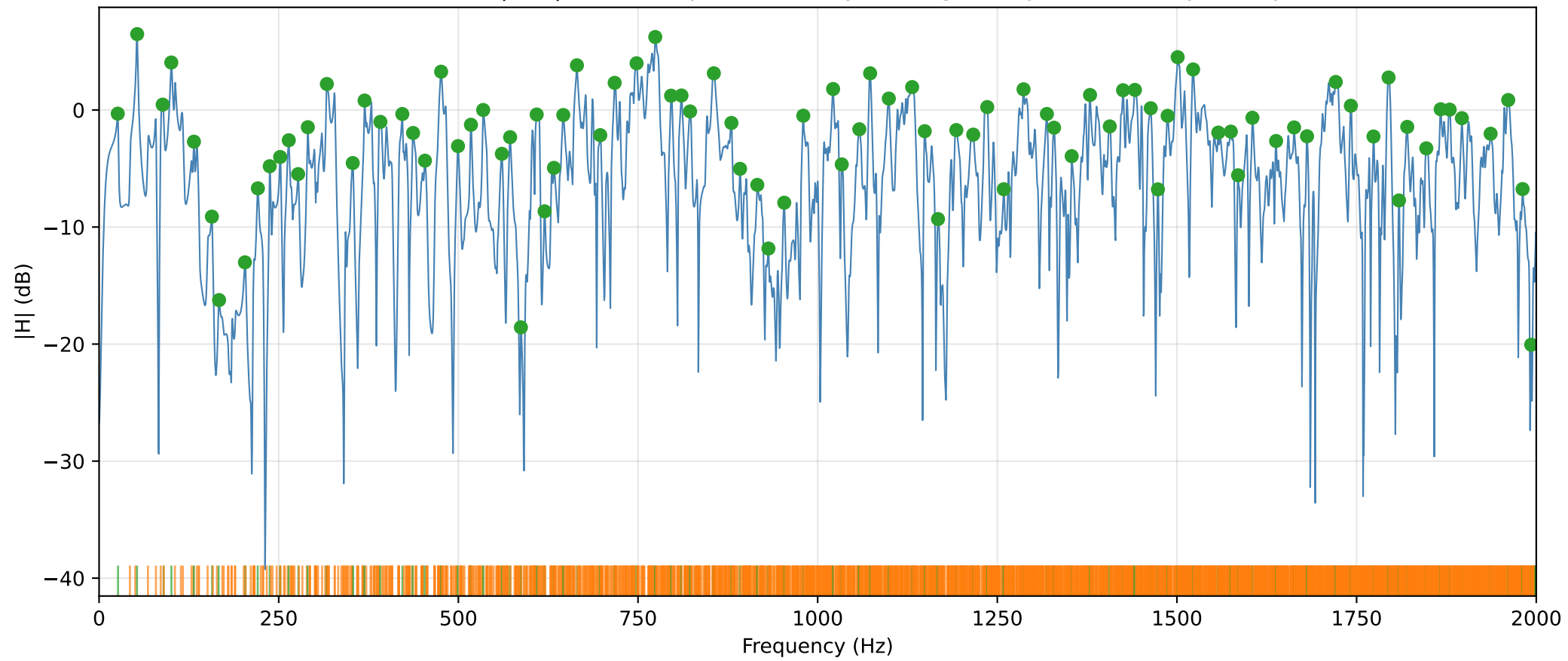
L=6.50 m — ISM |H(f)| with deduplicated analytical eigenfrequencies and picked peaks
