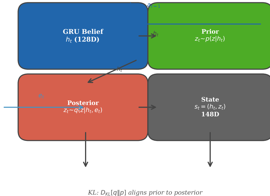
(b) World Model
