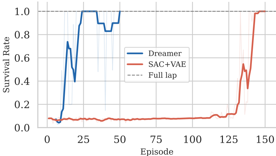
Survival Rate vs.\ Episodes
