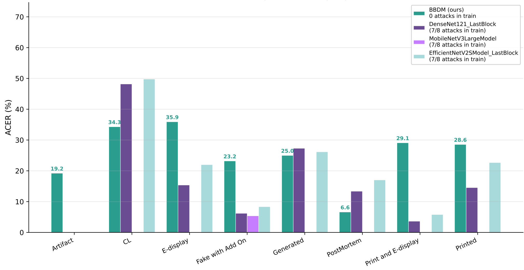
Per-Attack ACER: BBDM (Unsupervised) vs Top Supervised Models
