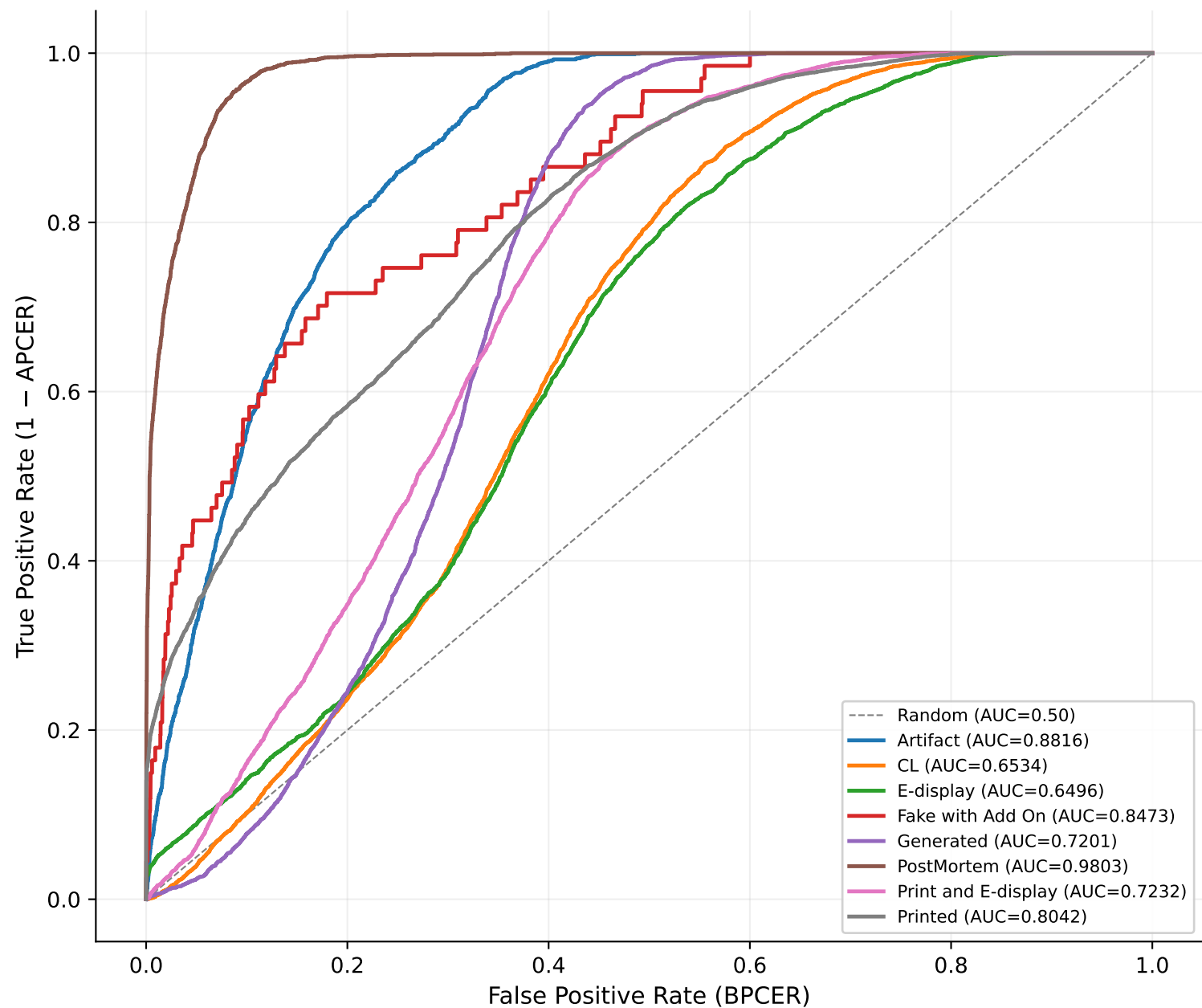
BBDM Leave-One-Out ROC Curves
