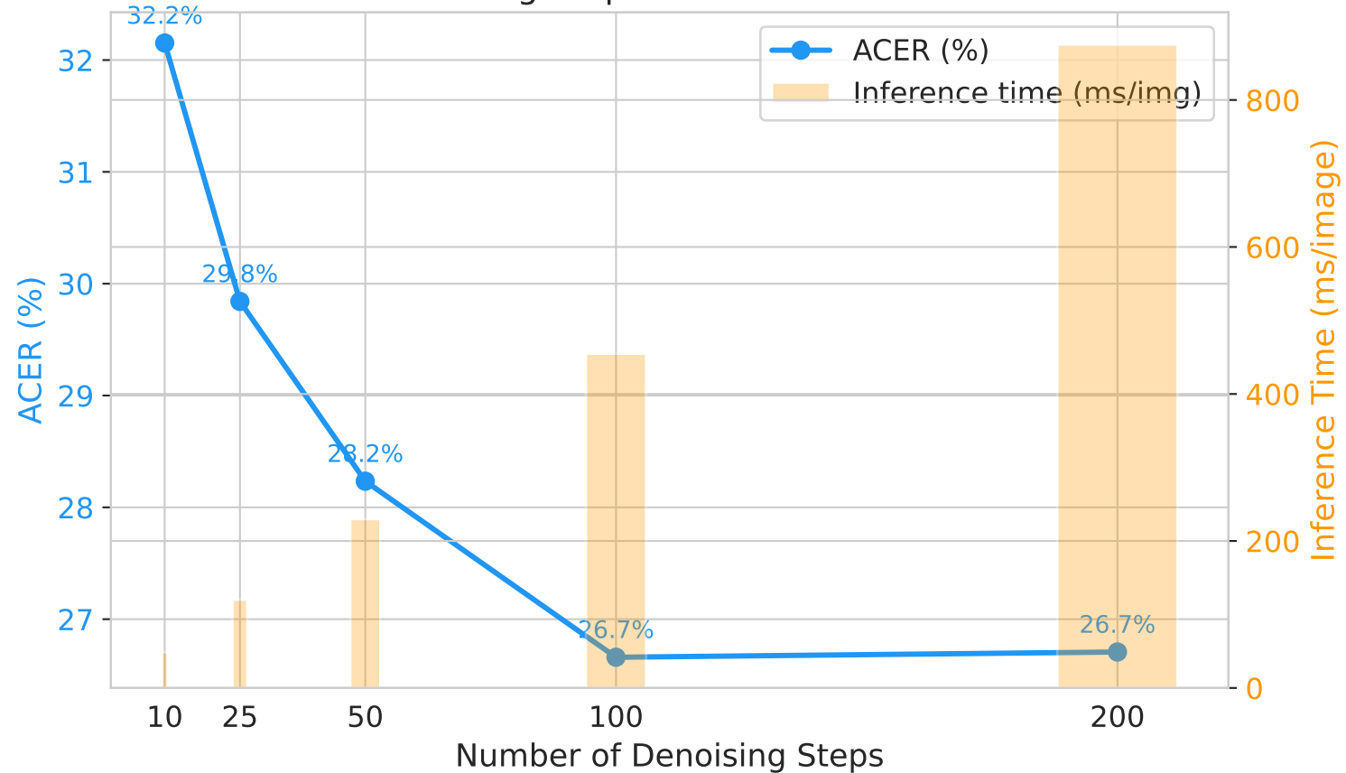
Ablation: Denoising Steps vs ACER and Inference Time
