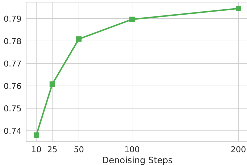
AUC vs Denoising Steps
