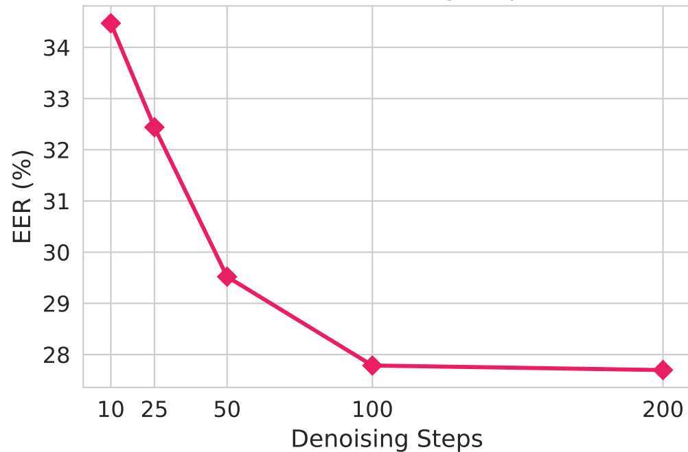
EER vs Denoising Steps
