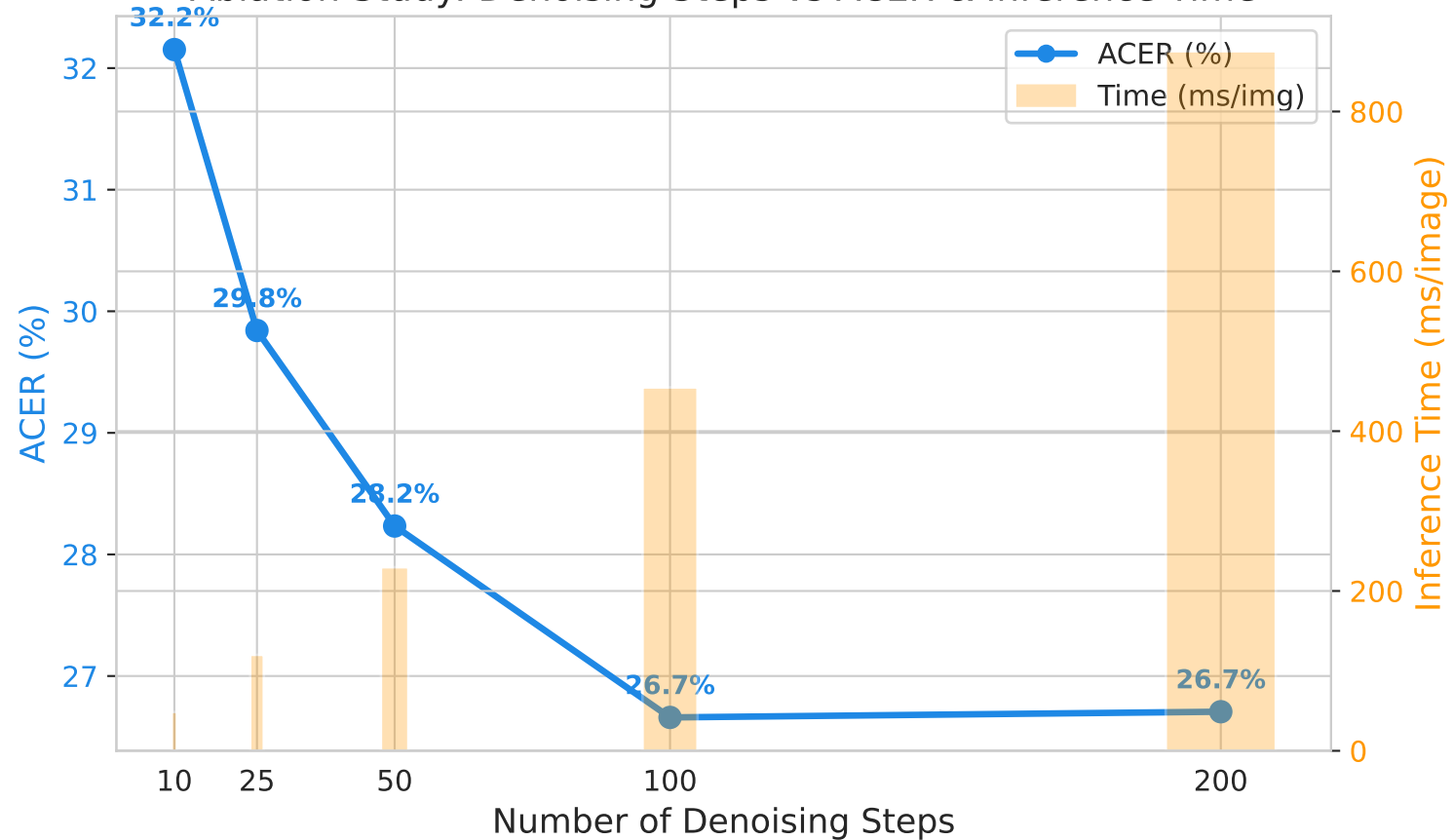
Ablation Study: Denoising Steps vs ACER & Inference Time
