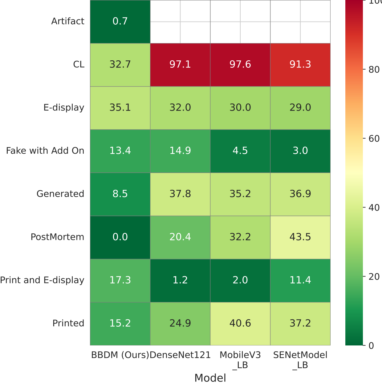
Per-Attack APCER (%) Heatmap: BBDM vs Supervised Baselines
