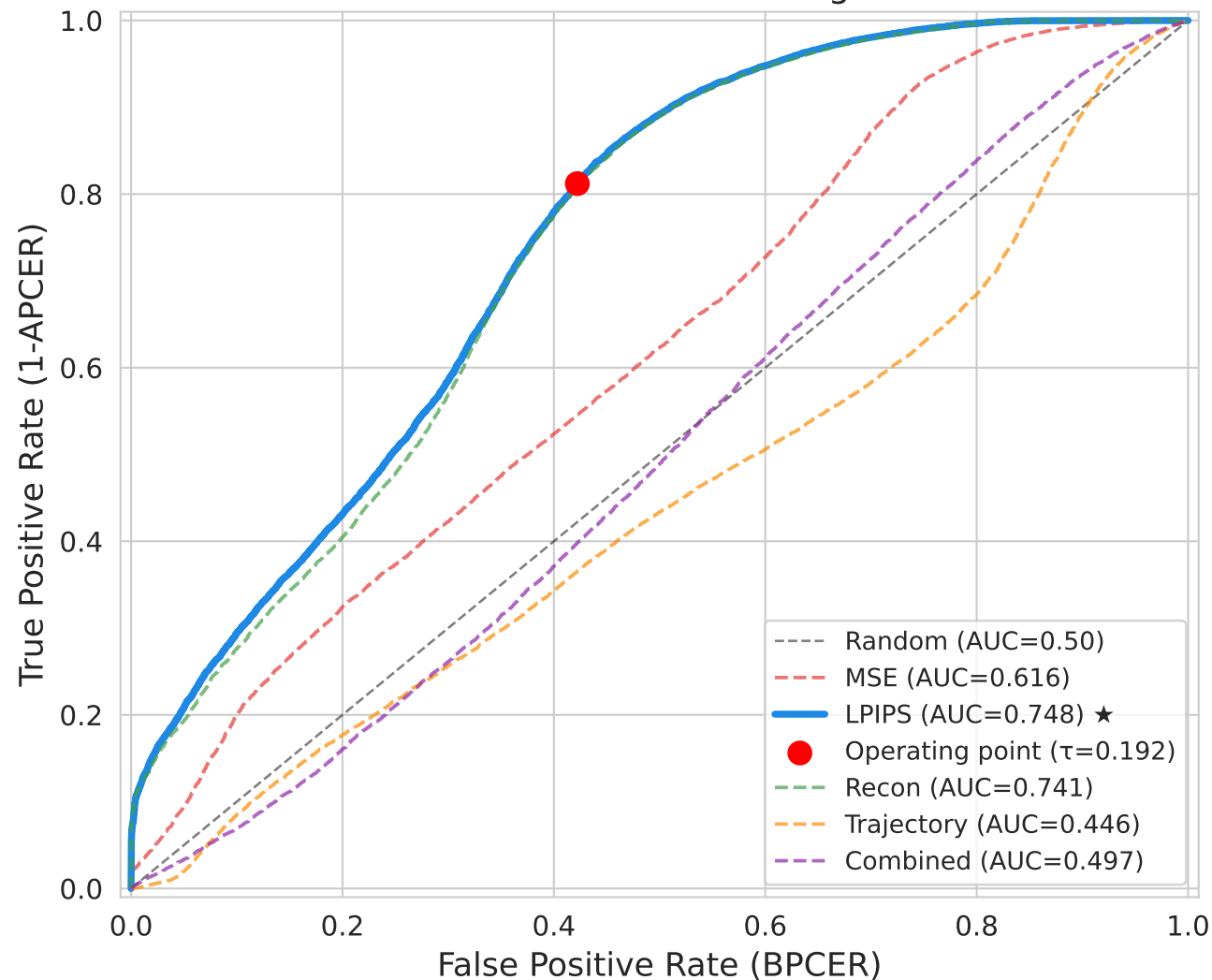
ROC Curves — Iris PAD Scoring Methods
