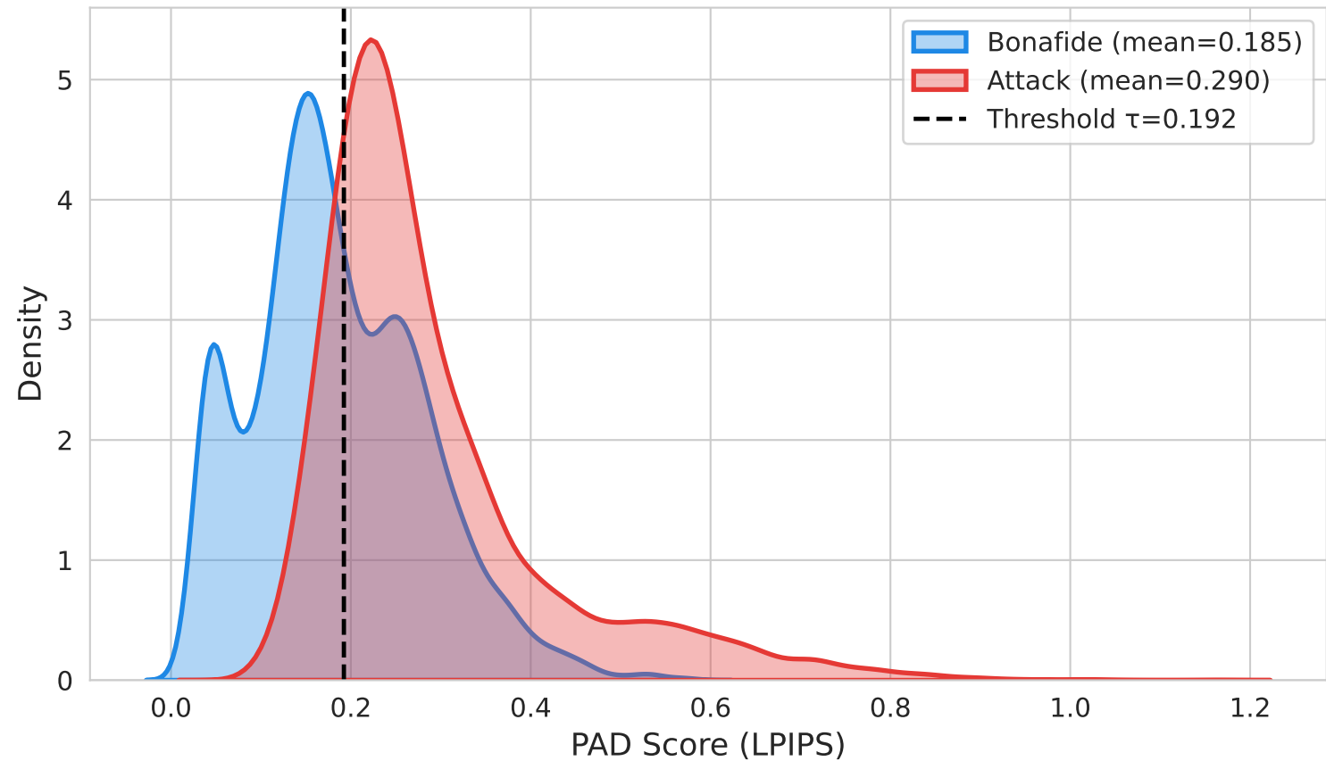
PAD Score Distributions: Bonafide vs Attack
