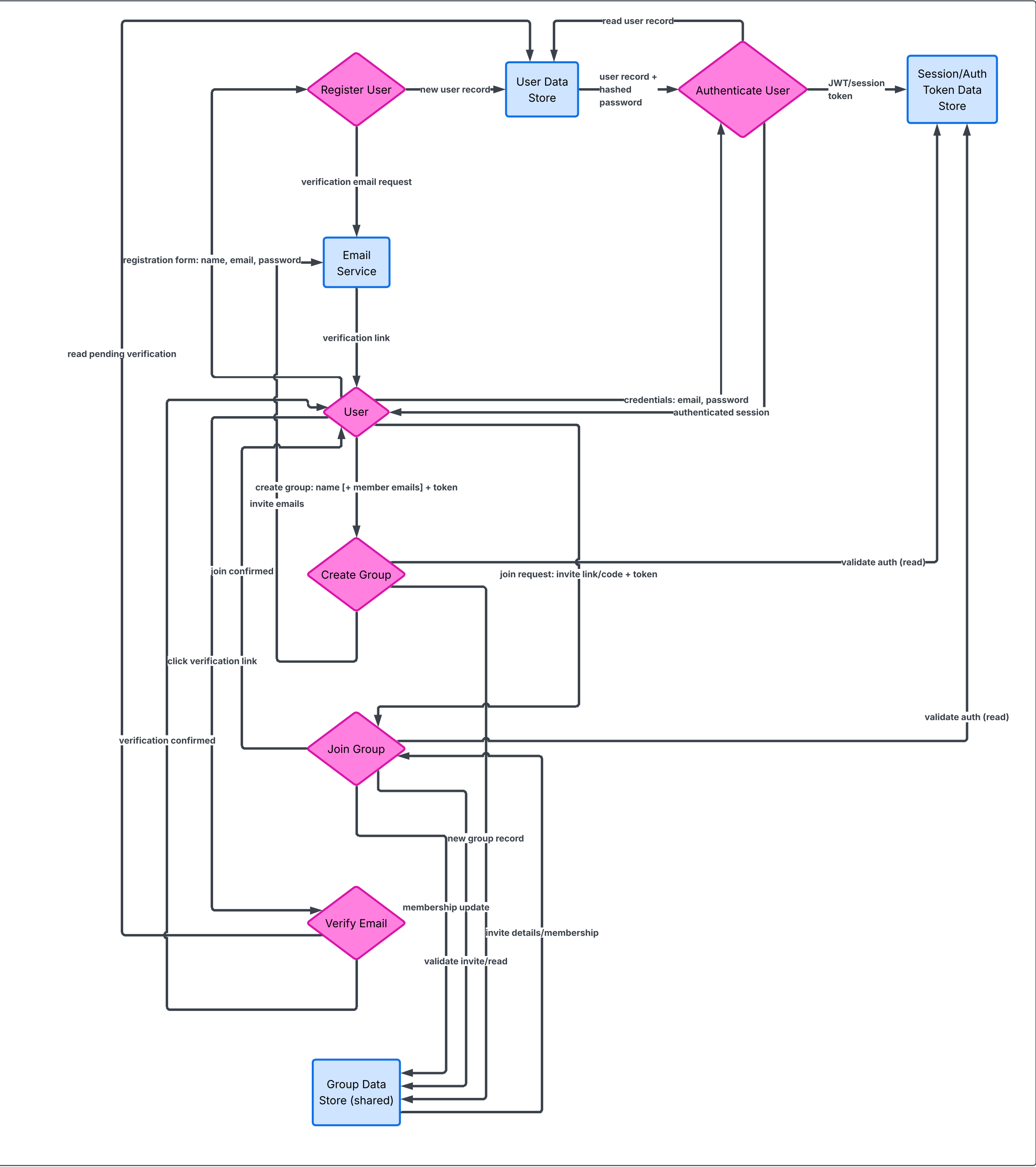
Authentication & Group Management DFD (Diagram 1)
