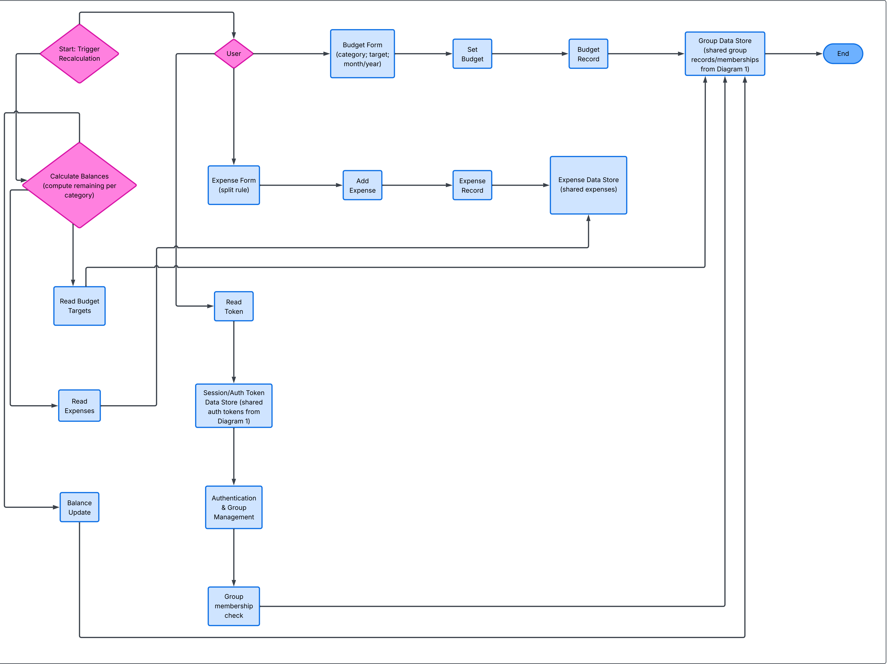
Spending vs. Target Calculation DFD (Diagram 2)
