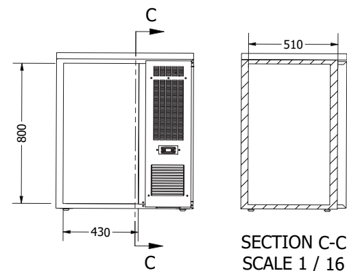
Inside dimensions 780
