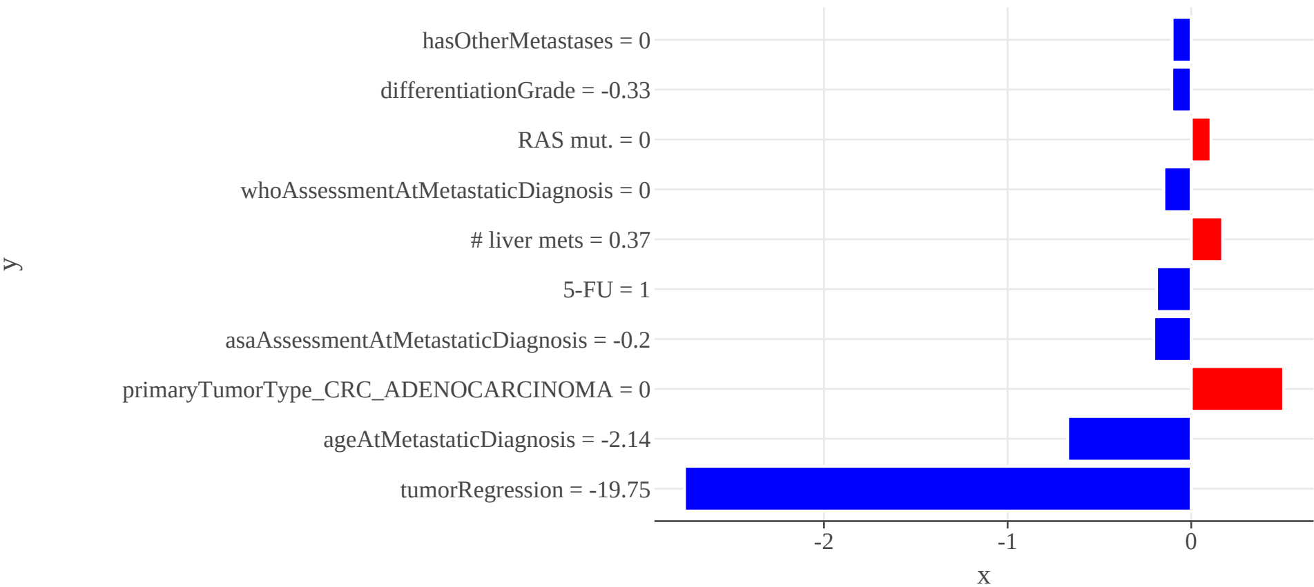
SHAP values for treatment: FOLFIRI
