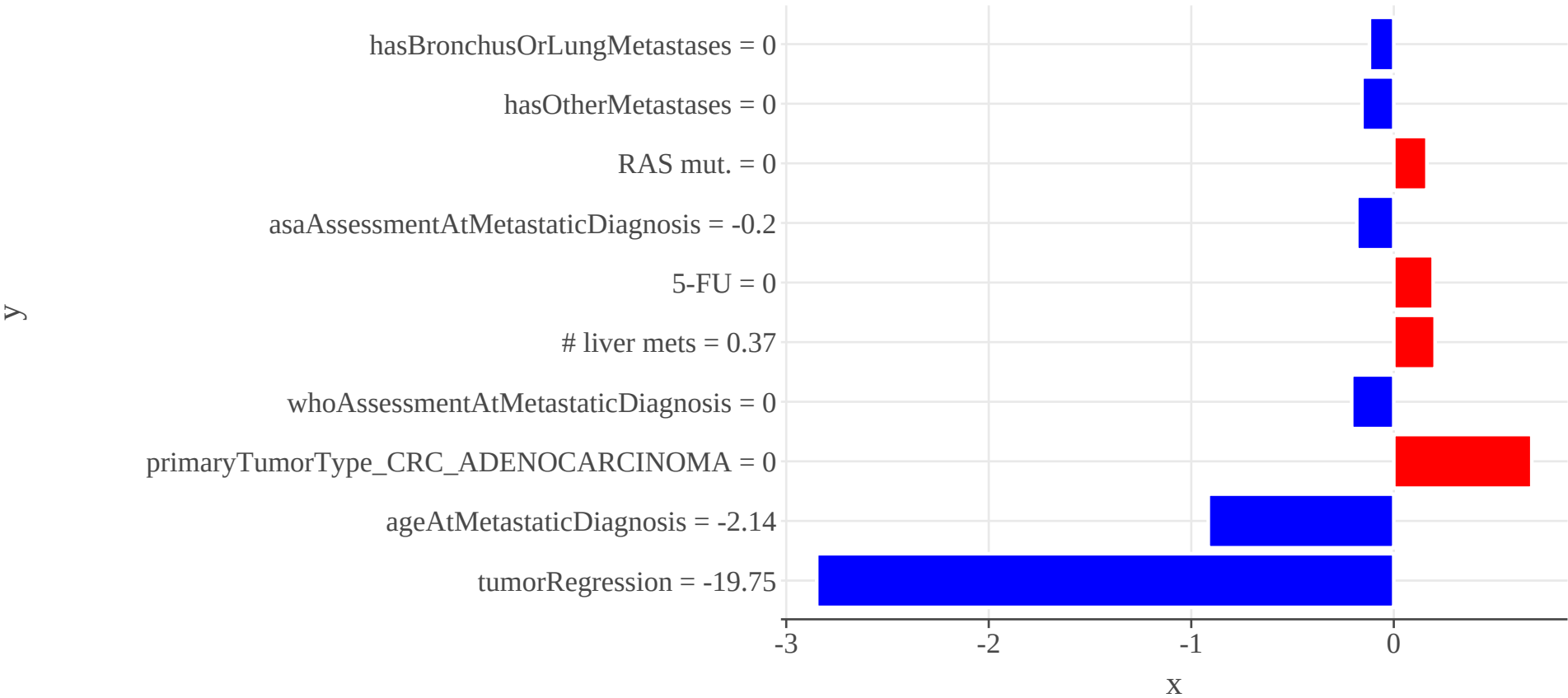
SHAP values for treatment: No Treatment
