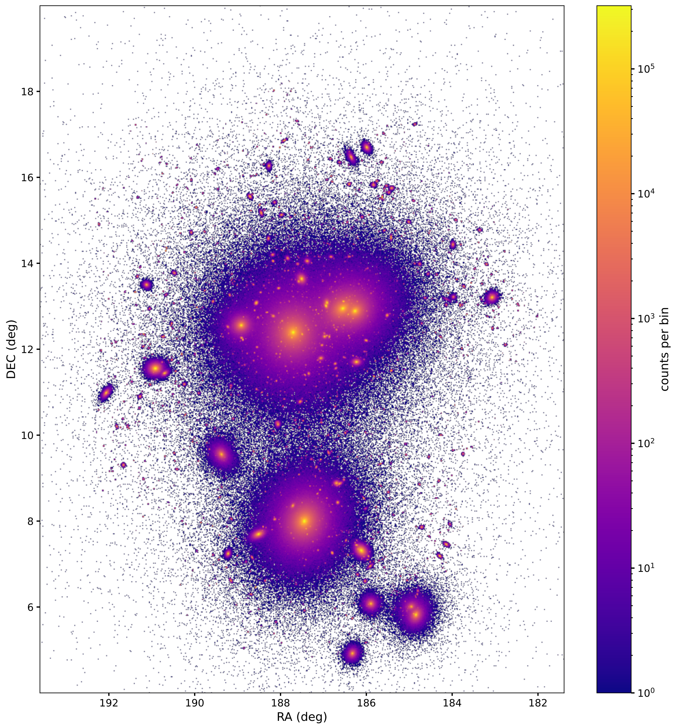
Virgo Cluster (3.6 arcsecond resolution)
