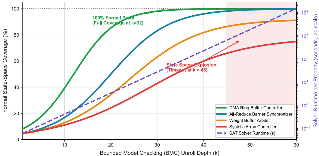
SystemVerilog Assertion Coverage vs. BMC Unroll Depth in Accelerator Units
