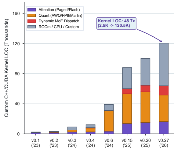
C. Inference Engine (vLLM) Application Kernel Fragmentation
