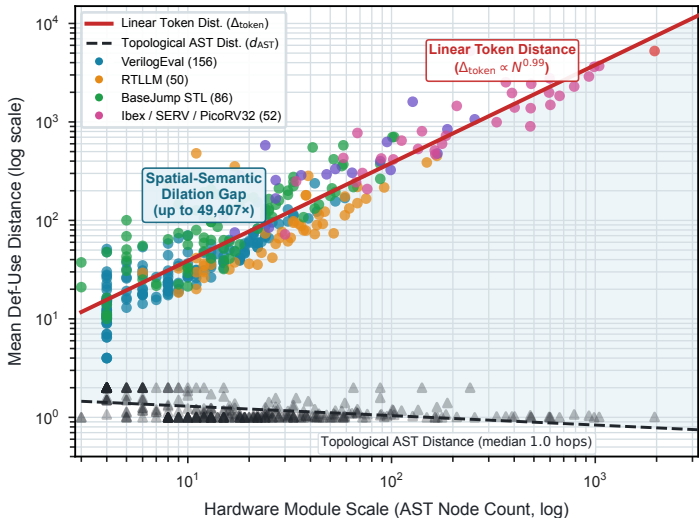
A. Spatial-Semantic Dilation (Def-Use Distance)
