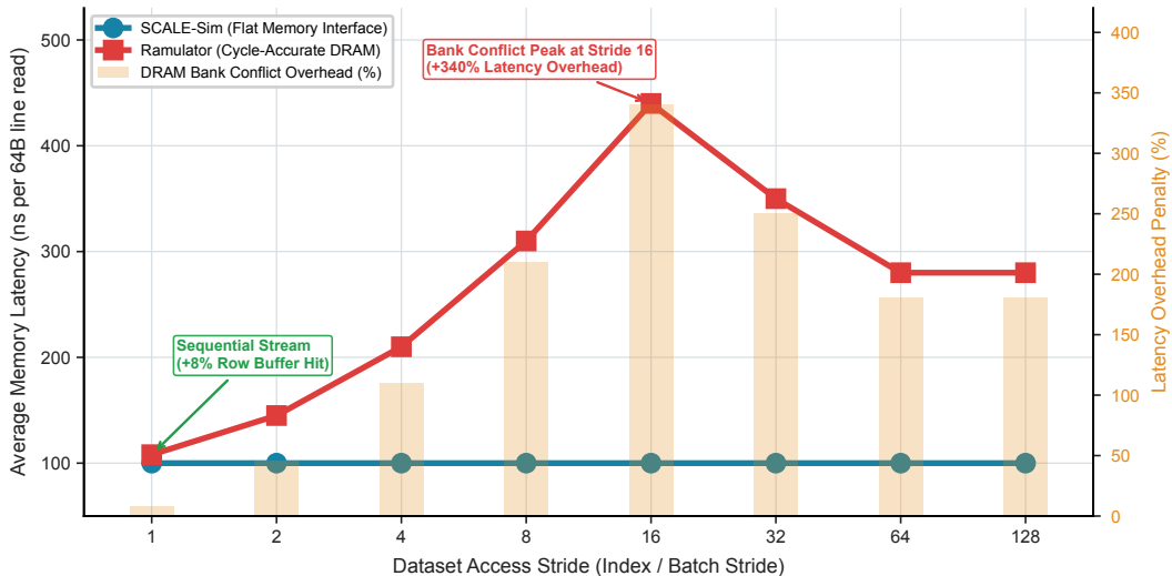
SCALE-Sim vs. Ramulator DRAM Bank Conflict Overhead across Access Strides
