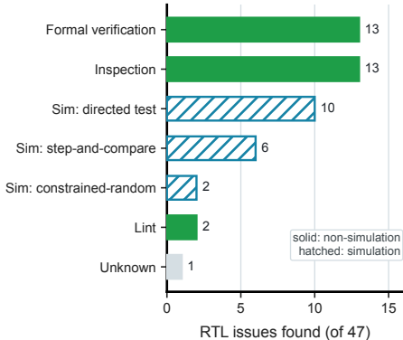
CV32E40P issues by finding method
