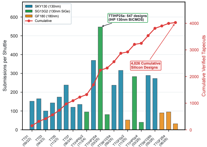
(b) Open Silicon Submission Renaissance
