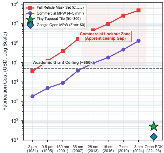
(a) Physical Silicon Fabrication Cost Barrier
